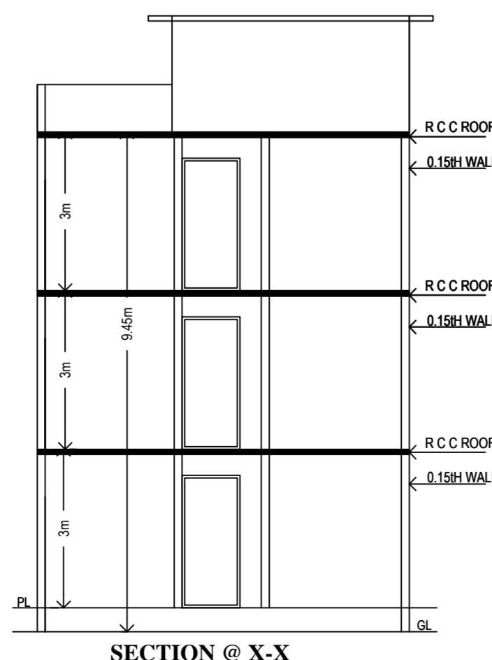
SECTION @ X-X
